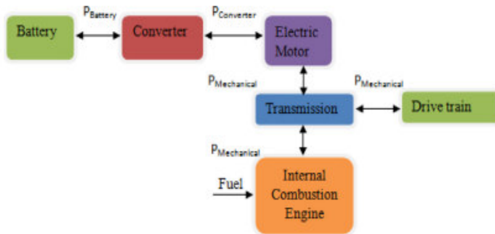
Figure 2. Power flow of parallel HEV
